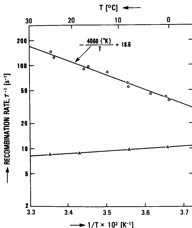
FIGURE 9 Temperature dependence of the charge recombination kinetics in RCs reconstituted in liposomes (see Fig. 8). The primary acceptor was either UQ ( \Delta ) or AQ ( \circ ). The solid lines for the AQ sample represent the theoretical fit: \ln \tau^{-1} = -4060(K)/T + 18.6 .
